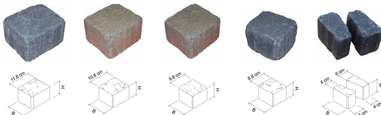
Pavés FRIEDA® 4/6 x 9.8 x 7 cm (pavés de calage)
